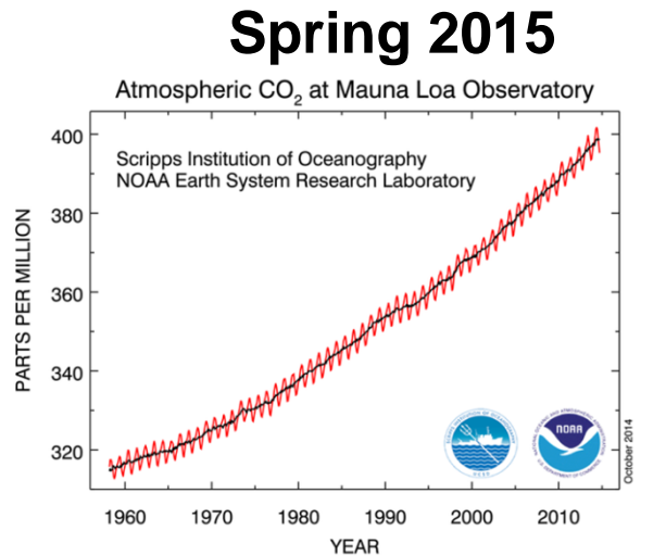
Current growth of CO 2 in the atmosphere.
